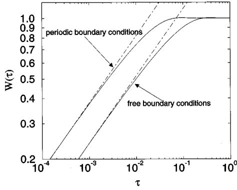
FIG. 3. Scaling function W(\tau) for the interface width in a system of finite size L for periodic boundary conditions and free boundary conditions, respectively. The dashed lines are approximations for small scaled times \tau = \lambda C_L t L^{-3/2} , W(\tau) \approx 3.8\tau^{1/3} for periodic boundary conditions and W(\tau) \approx 2.4\tau^{1/3} for free boundary conditions.
