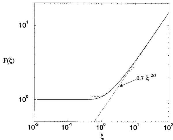
FIG. 2. Scaling function F(\xi) for the truncated correlation function in real space versus the scaling variable \xi = \lambda A^{1/2} t / x^{3/2} . The empirical forms, Eq. (3.50), are shown as the dashed curves. The dimensionless coupling constant can be read off from the crossover point of F(\xi) .
