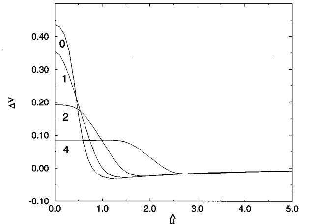
FIG. 5. Real part of the vertex correction \Delta V versus \hat{\mu} , where \Delta V = \text{Im}[\hat{\nu}(\hat{\mu} - \hat{\omega}/2) - \hat{\nu}(\hat{\mu} + \hat{\omega}/2)]/\hat{\omega} . The values of the scaling variable \hat{\omega} = 0, 1, 2, 4 are indicated in the graph.
