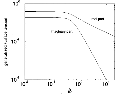
FIG. 4. Scaling function for the real part, \text{Re}[\hat{\nu}(\hat{\omega})] , and imaginary part divided by the scaled frequency, \text{Im}[\hat{\nu}(\hat{\omega})]/\hat{\omega} , of the generalized surface tension.
