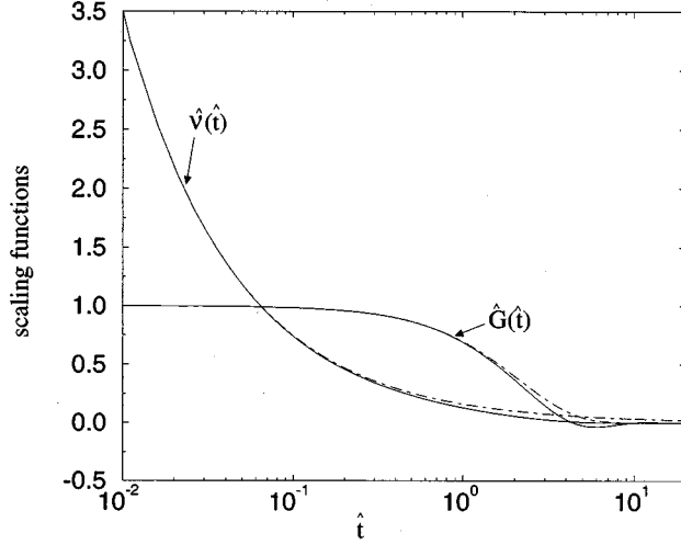
FIG. 1. Scaling functions for the generalized surface tension \hat{v}(\hat{t}) and response function \hat{G}(\hat{t}) vs the scaling variable \hat{t} = \lambda(D/\nu)^{1/2}k^{3/2}t . The point-dashed line represents the Gaussian approximation, Eq. (3.46), for the response function, which is obtained from the analysis of the mode-coupling equations at small times.
